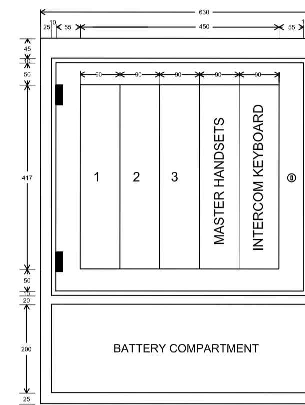
FRONT VIEW ( INTERNAL DETAIL )
