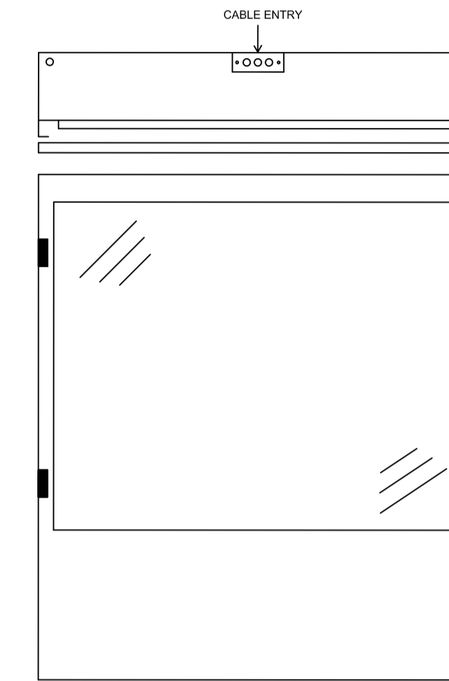
( DOOR ONLY ) FRONT VIEW
