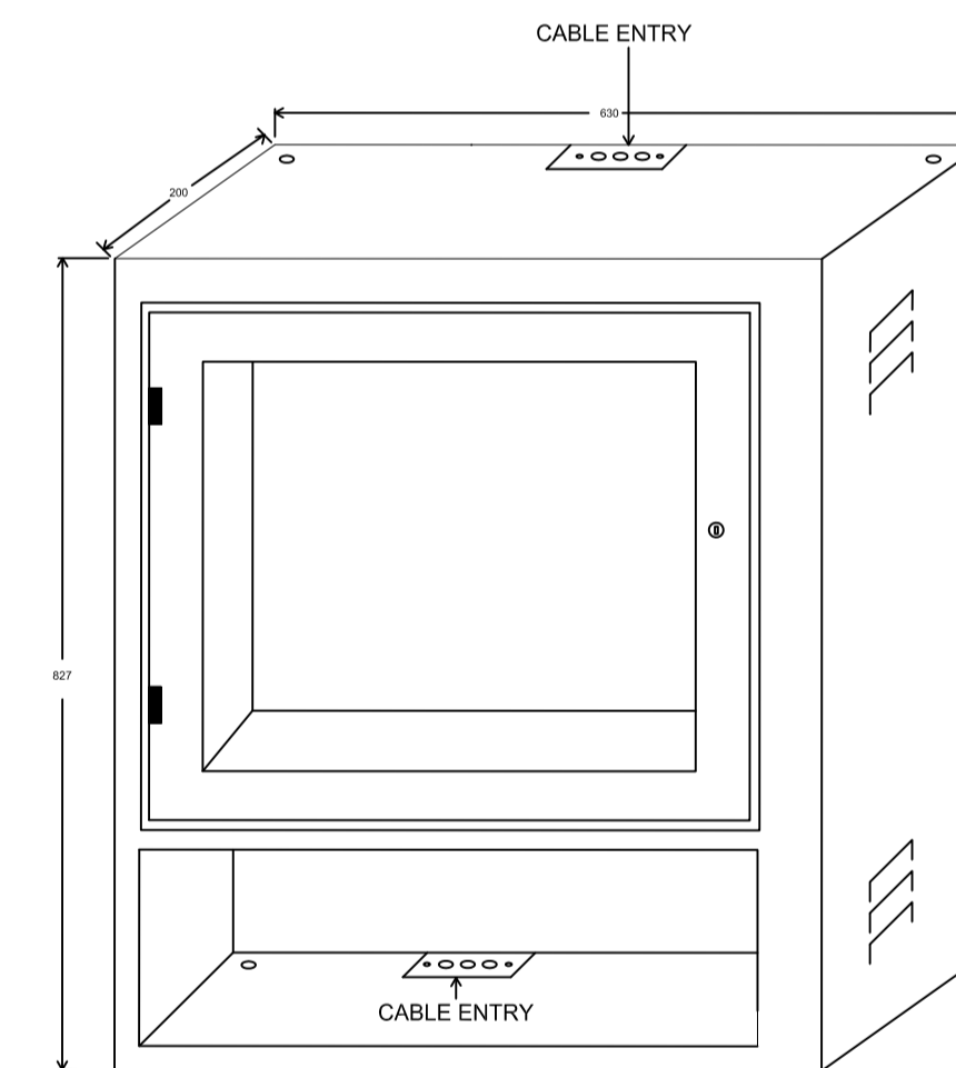
ISOMETRIC VIEW
