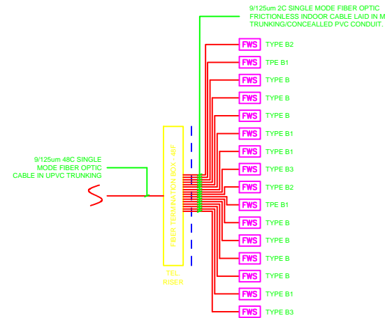
8TH FLOOR TEL RISER- BLOCK B SIMILAR TO 9TH FLR. UP-TO 26TH FLR BLOCK B
