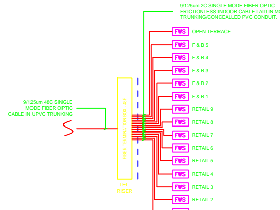
1ST FLOOR TEL RISER- RETAIL B
