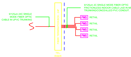
2ND FLOOR TEL RISER- RETAIL A
