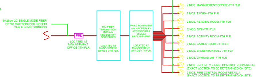
TELEPHONE SCHEMATIC FOR MANAGEMENT OFFICE (LEVEL 7)
