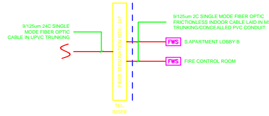
GROUND FLOOR TEL RISER- BLOCK A
