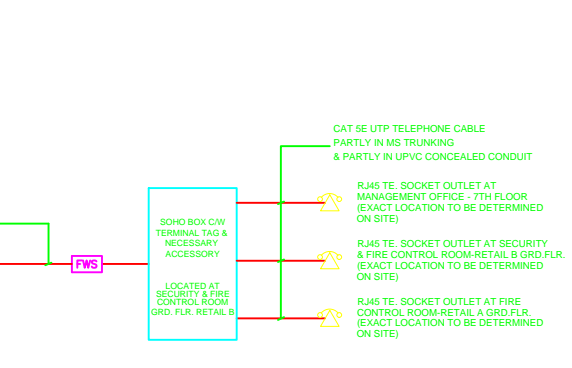
SECURITY & FIRE CONTROL ROOM
