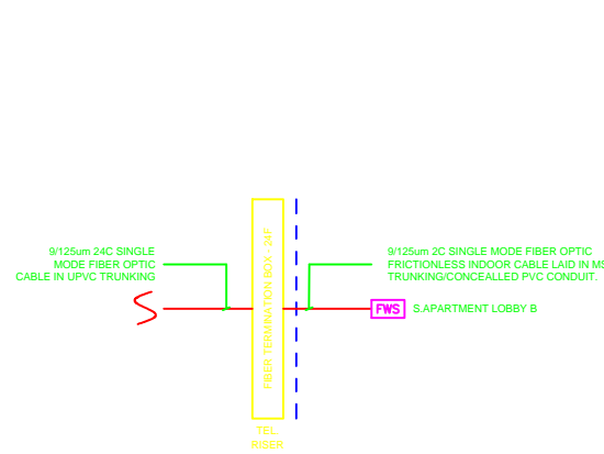
GROUND FLOOR TEL RISER- BLOCK B SIMILAR TO 7TH FLOOR -BLOCK B & BLOCK A
