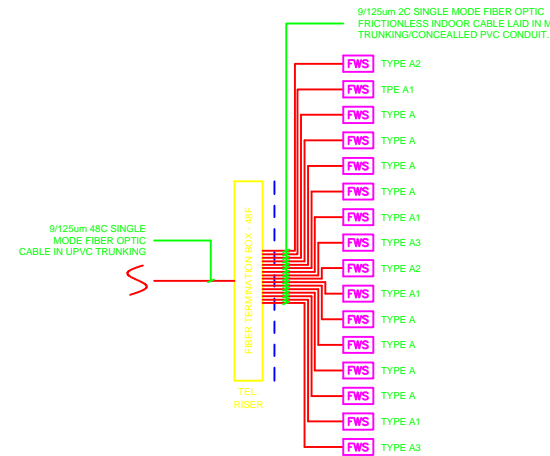
8TH FLOOR TEL RISER- BLOCK A SIMILAR TO 9TH FLR. UP-TO 26TH FLR BLOCK A
