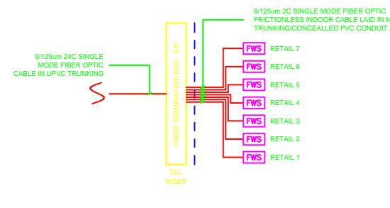
1ST FLOOR TEL RISER- RETAIL A
