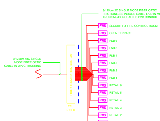
GROUND FLOOR TEL RISER- RETAIL B SIMILAR TO 3RD FLOOR- RETAIL B
