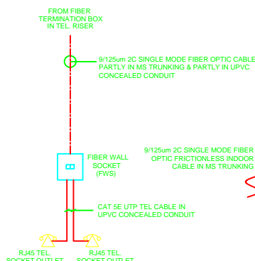
TYPICAL DETAIL FOR S.APARTMENT
