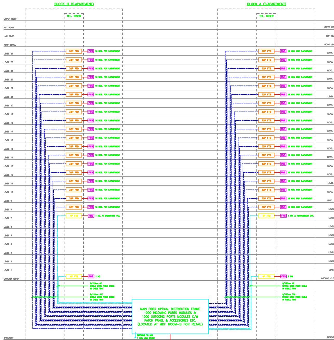
TELEPHONE SCHEMATIC TOWER A & B
