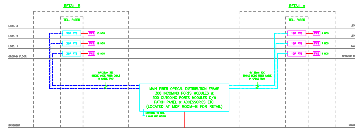
TELEPHONE SCHEMATIC RETAIL (COMMERCIAL)
