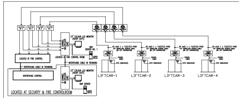
LIFT ACCESS FOR BLOCK A SIMILAR WITH BLOCK B (RESIDENTIAL BLOCK)
